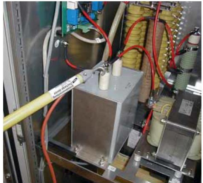
Single-pole device for discharging static charges
