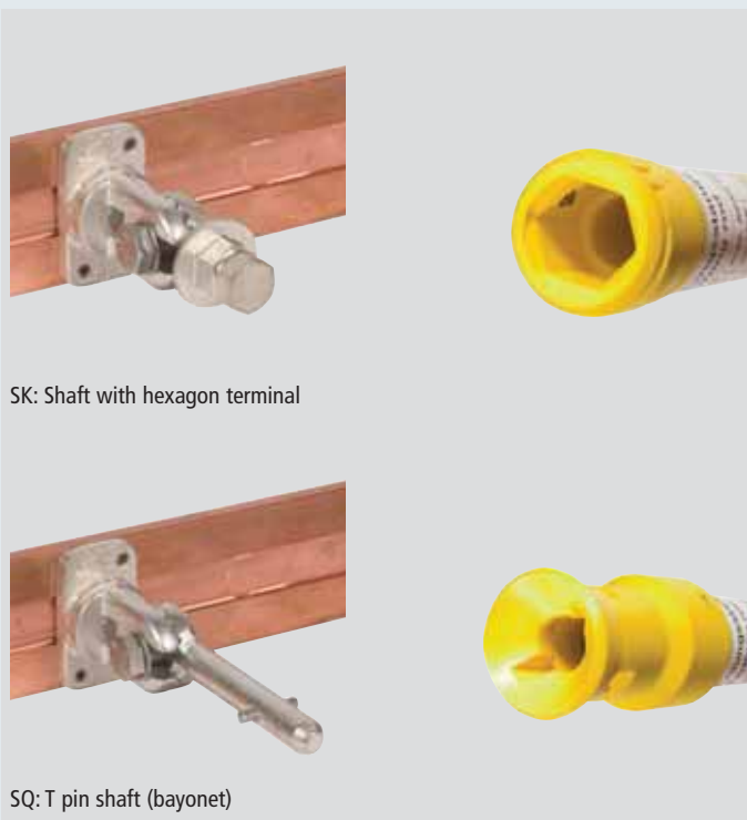
SK: Shaft with hexagon terminal
